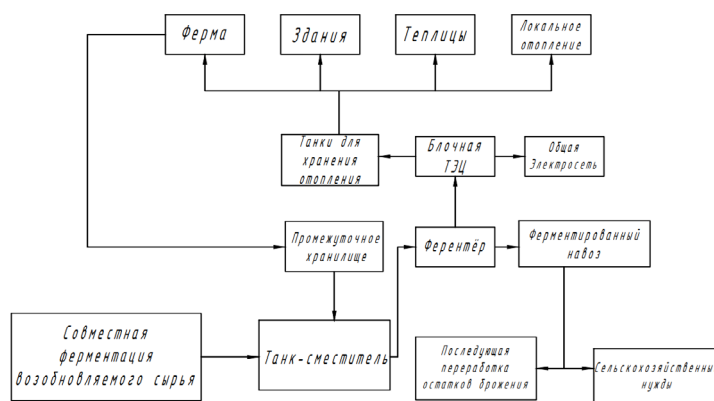
Figure 3 – Biogas production technology
